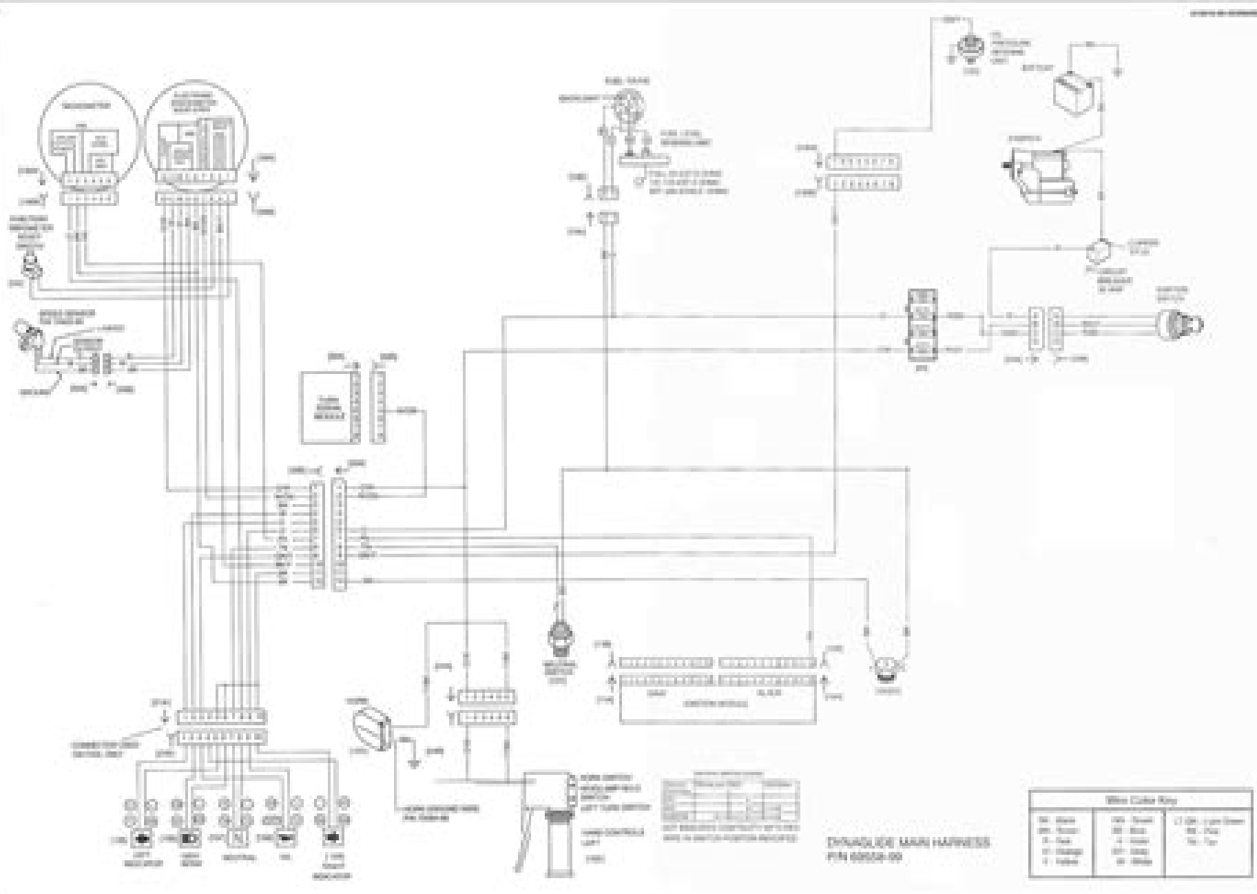
DYNA GLIDE WIRING DIAGRAM (Domestic and International Models), Horn and Instruments
