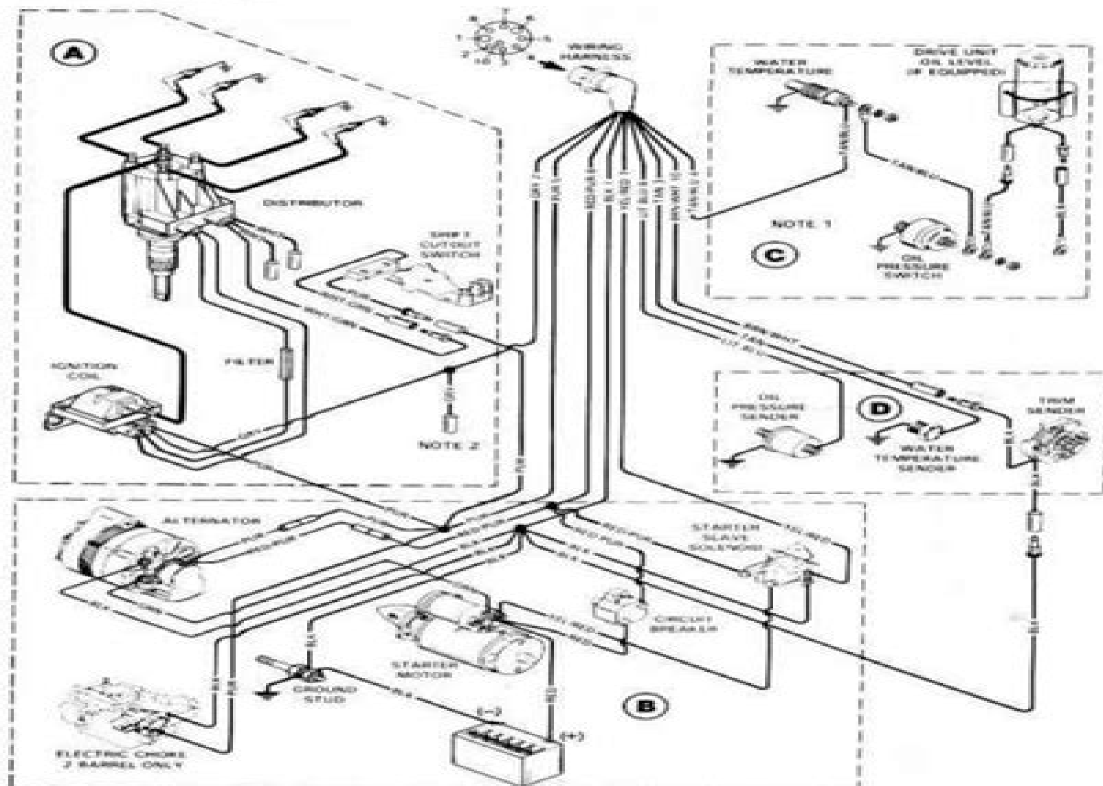
A: Ignition and Choke System B: Starting and Charging System
