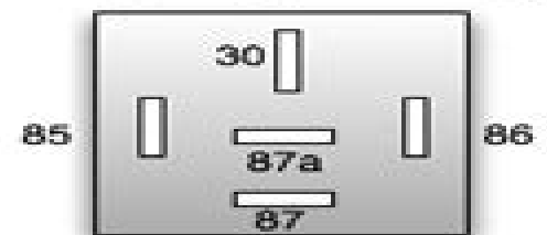
40 amp relay pin markings
