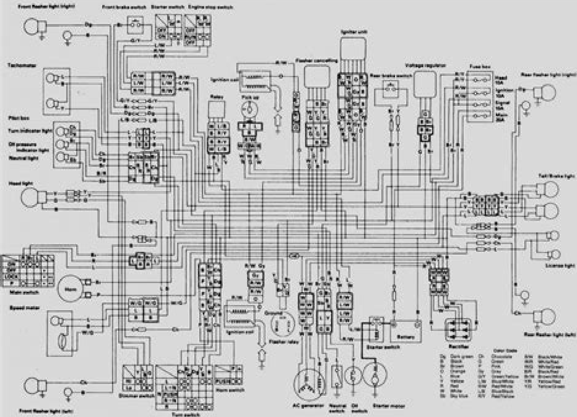
XS400Q/50, 1981 models
