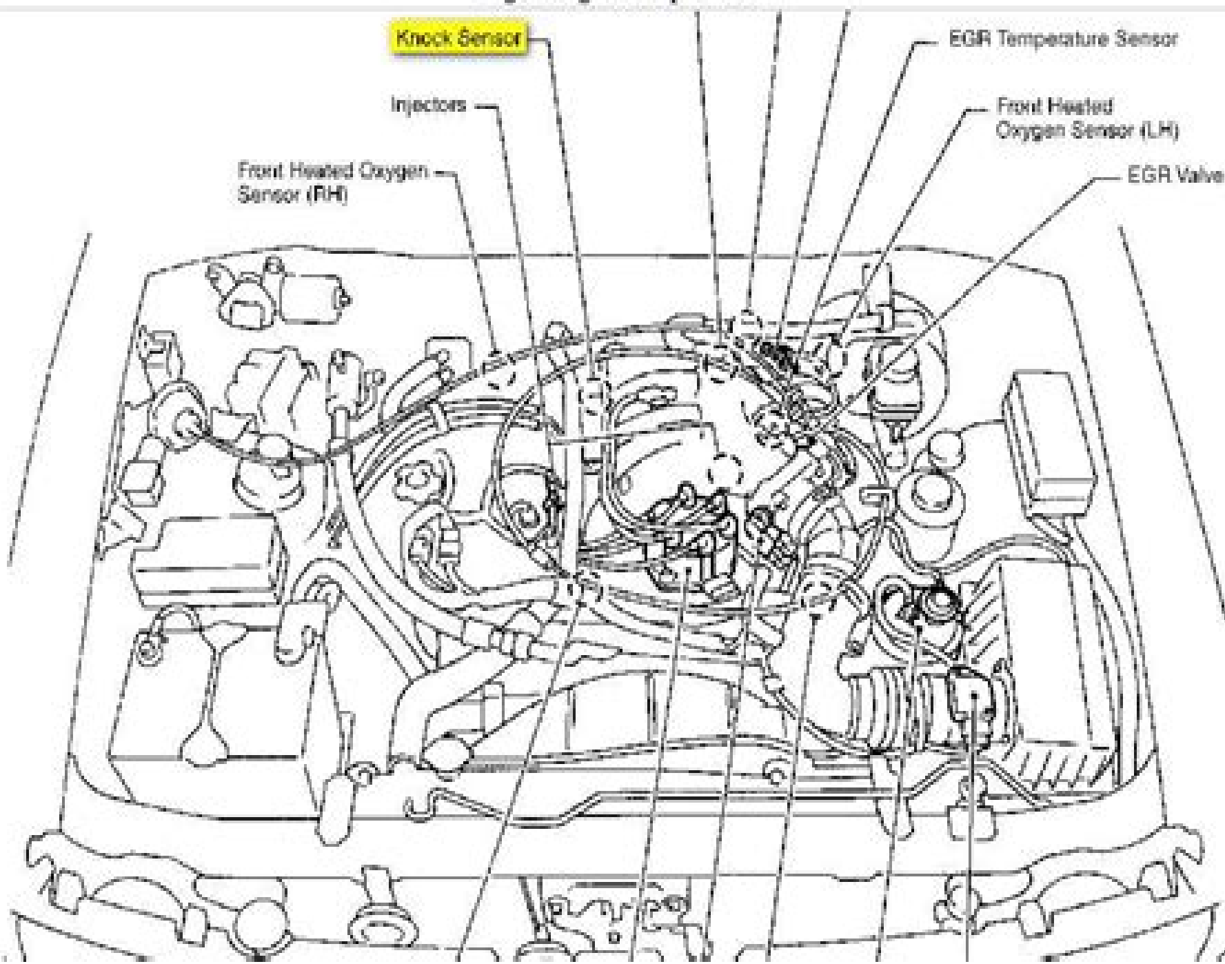
Fig. 2: Engine Compartment
