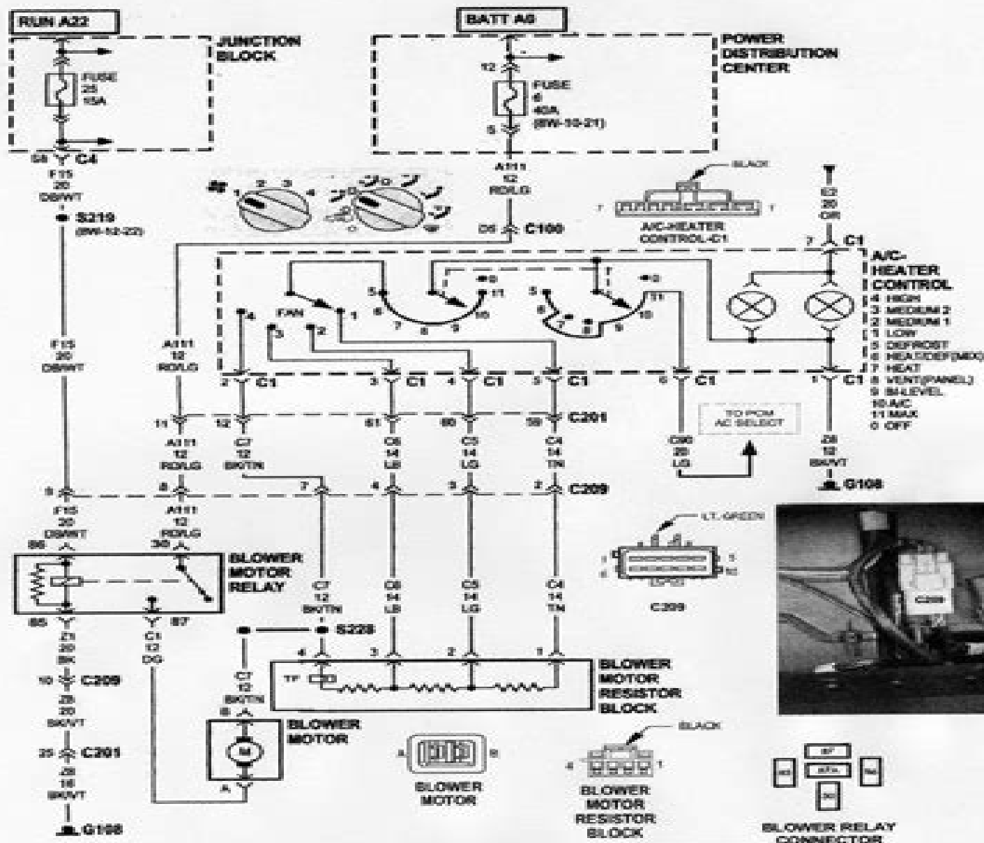
1997 - 2001 XJ HVAC BLOWER CIRCUIT
