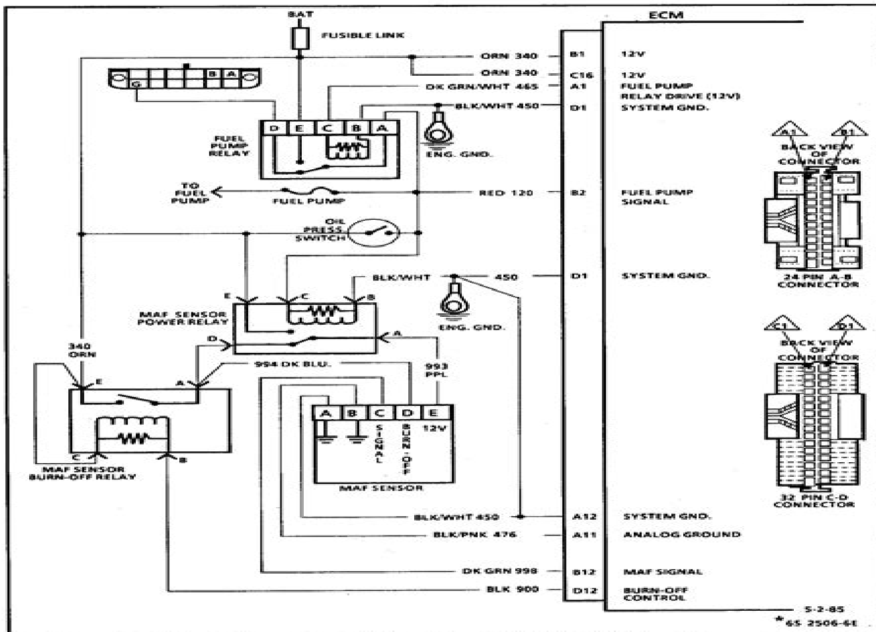
Figure A-4 - 5.7L, Wiring Diagram "Y" Series (3 of 4)
