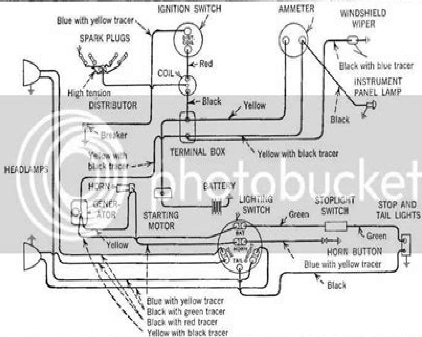
Fig. 28.—Wiring Diagram of the Ford Model A Showing All Units and Connections.
