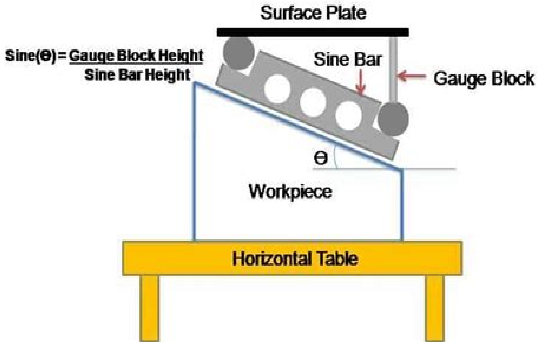
Principle of Sine Bar
