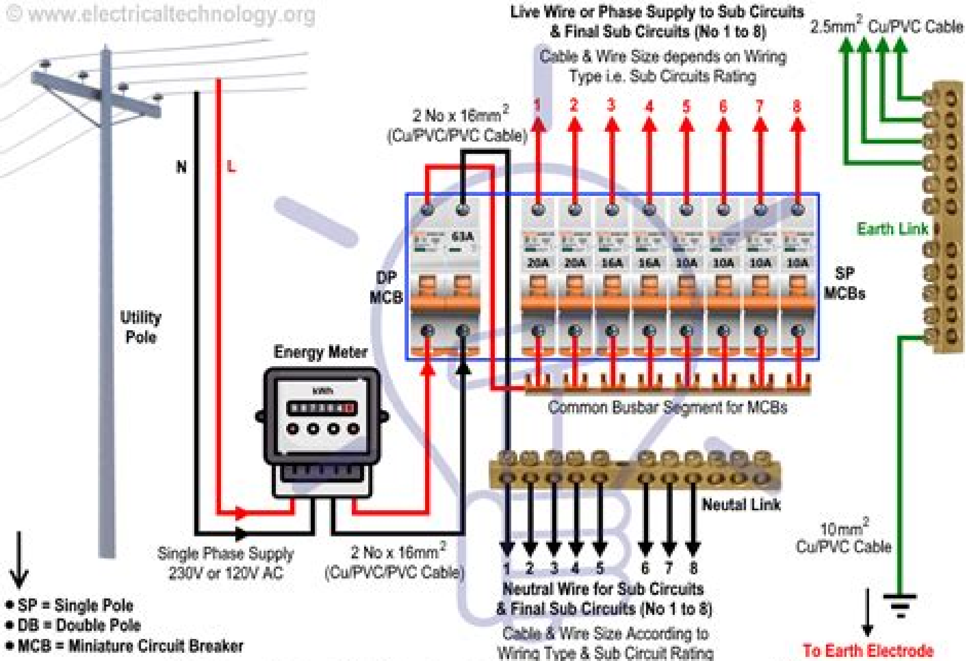
Wiring of the Distribution Board (Single Phase Supply) (From Utility Pole & Energy Meter to the Consumer Unit)
