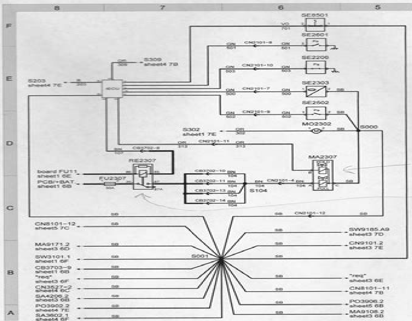
Figure 1 Wiring diagram 2
