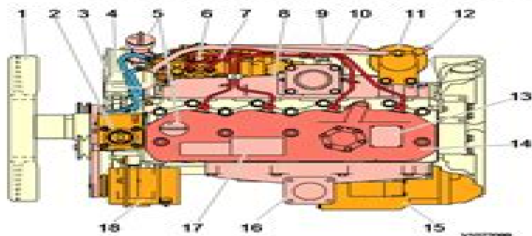
Figure 1 Engine, top side view
