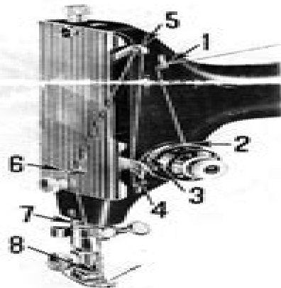
Fig. 2. Upper Threading
