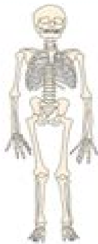
skeleton
