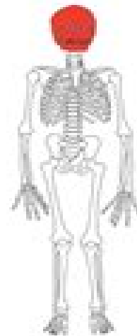
skull
