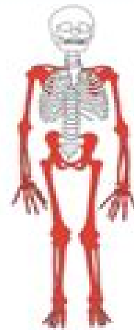
appendicular skeleton
