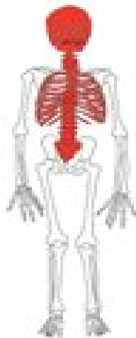
axial skeleton
