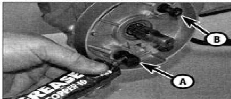
12.6 Lubricate the cam (A) and pivot pin (B) with a smear of grease
