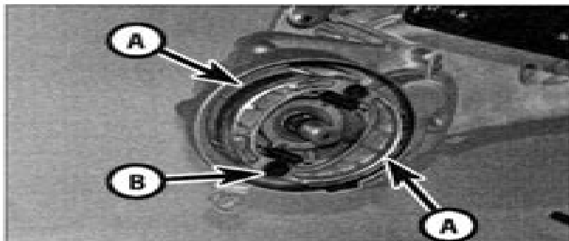
11.3 Check the friction material on the brake shoes (A). Note the brake cam (B)
