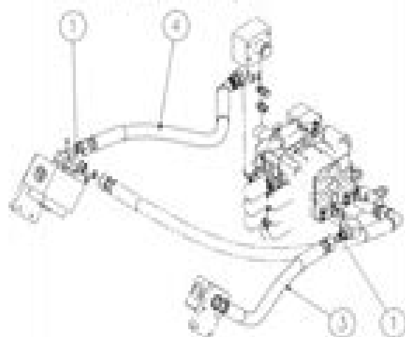
Fig. 21. Hose installation
