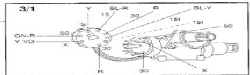
Ignition switch
