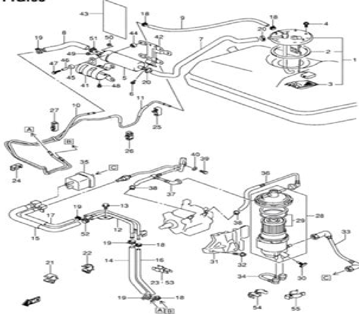
SO420W-2 E22_065 FUEL PUMP (420WD-RH2)
