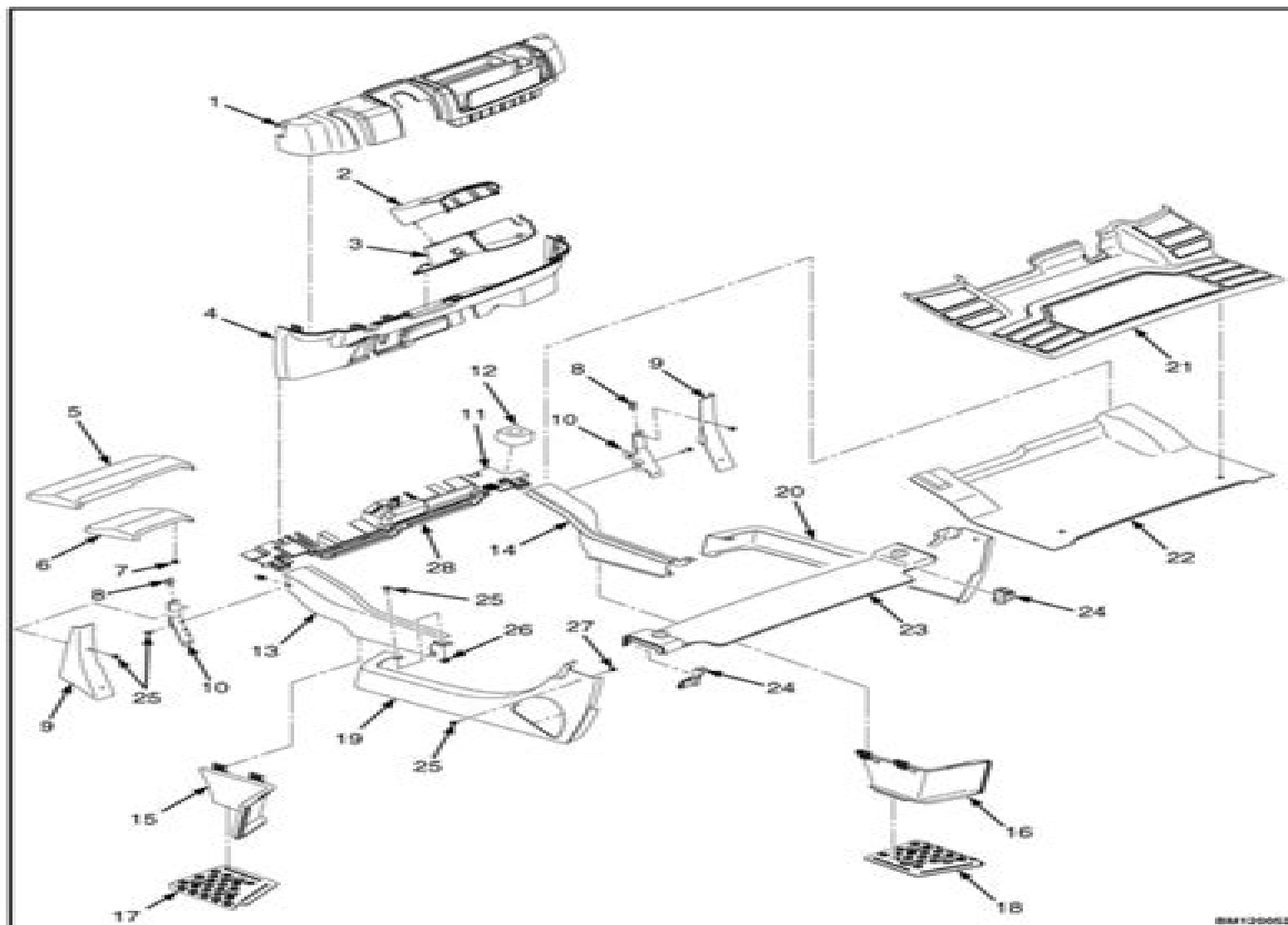
Figure 4. Side Covers, Floor Plate, and Cowl Components GLP/GDP20-35VX (GP/GLP/GDP040-070VX) (C875)
