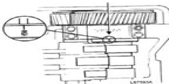
Fig. 150 Camshaft marking
