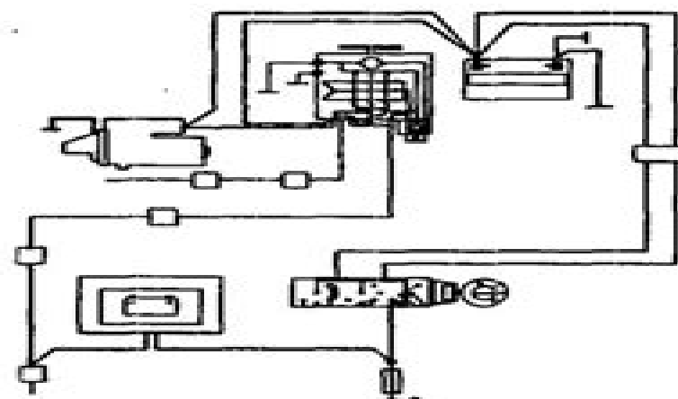
Alternator charging
