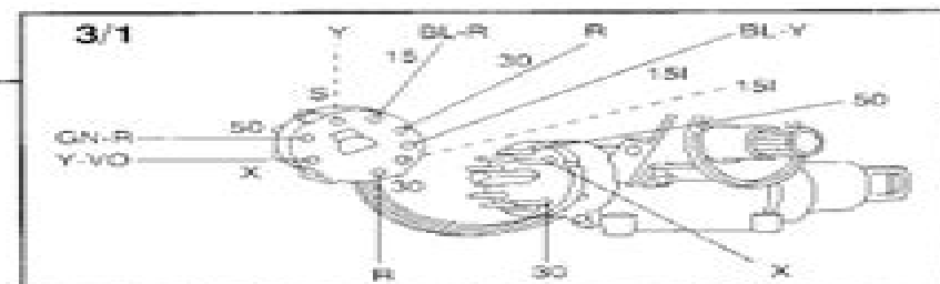
Ignition switch
