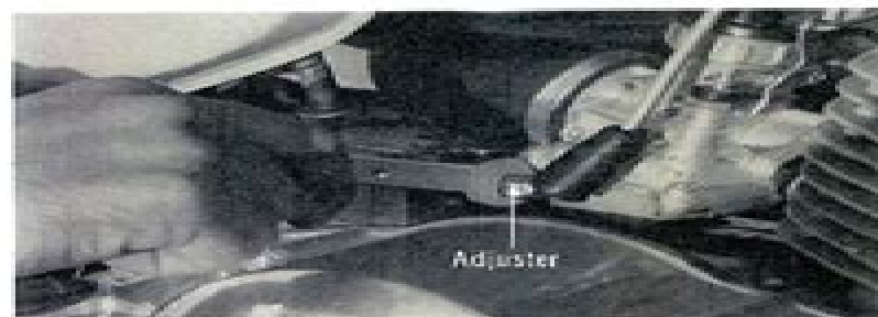
Fig. 6-5-4 Adjusting oil pump control cable
