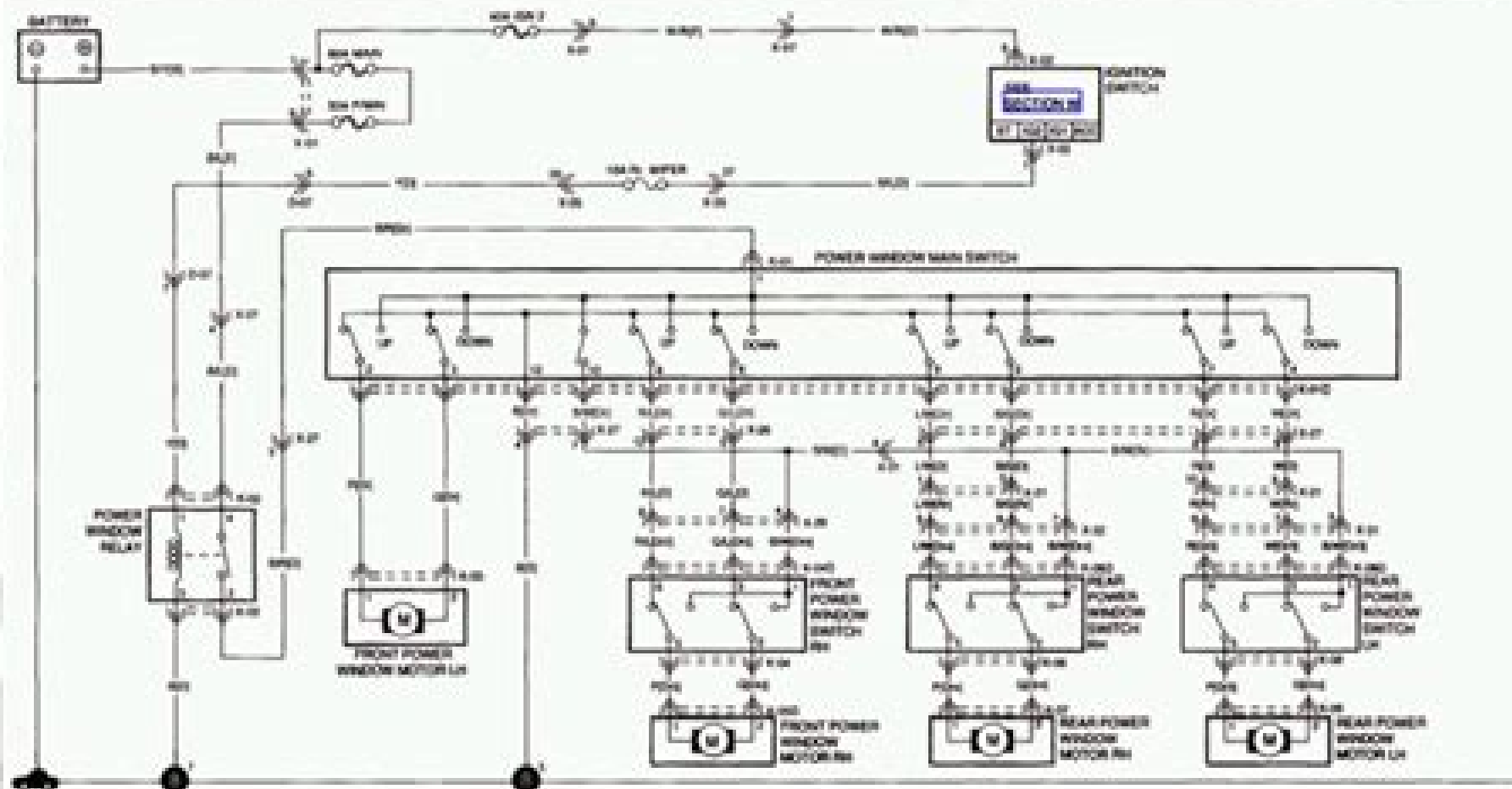
K-01 POWER WINDOW MAIN SWITCH (24)
