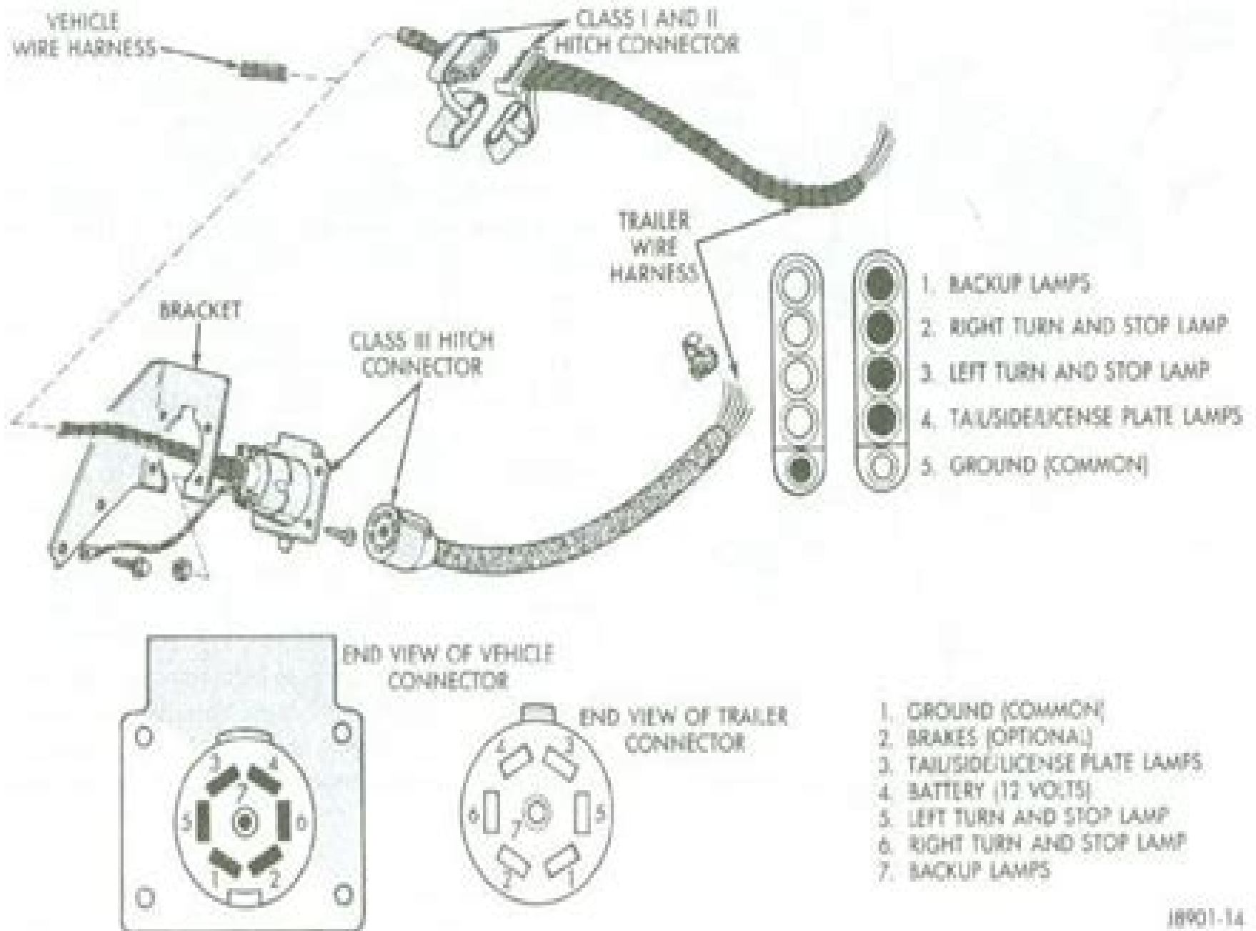
Fig. 14 Trailer Wire Harness Connectors
