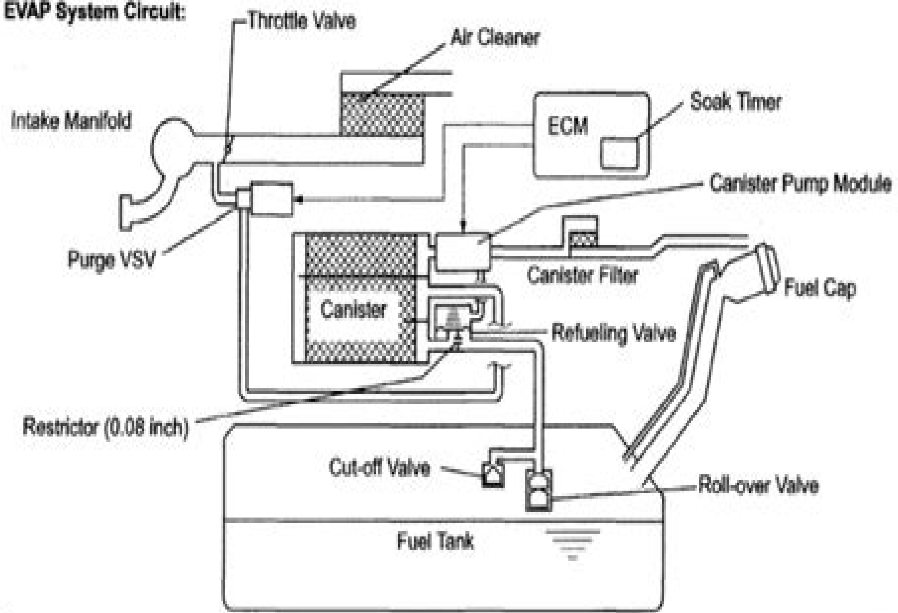
Fig 2: Identifying EVAP System Diagram
