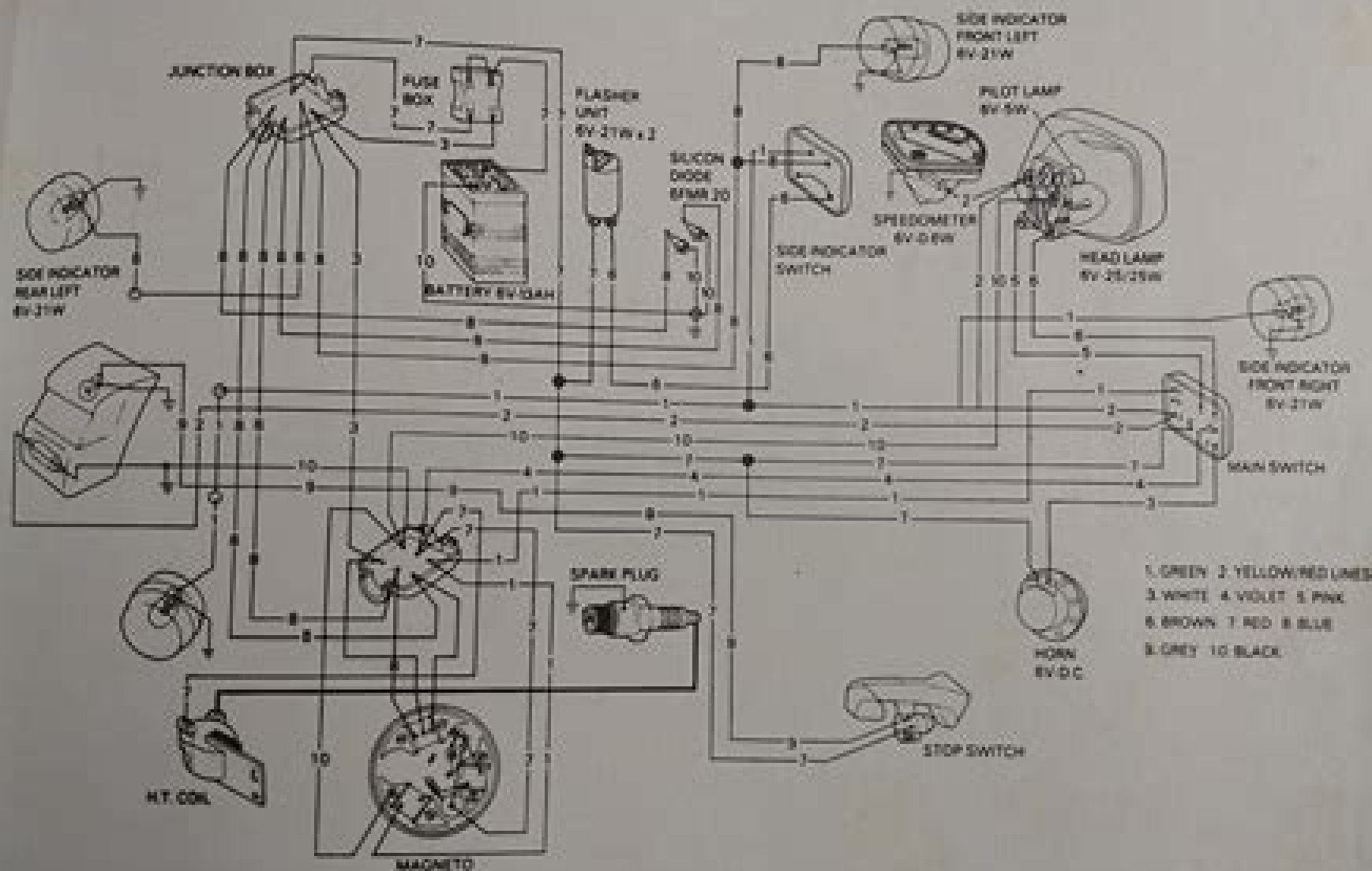
Fig. 21 (e) Wiring diagram for bajaj-Chetak with D. C. Blinkers (also applicable for bajaj-Super except the change in shape of tail lamp)
