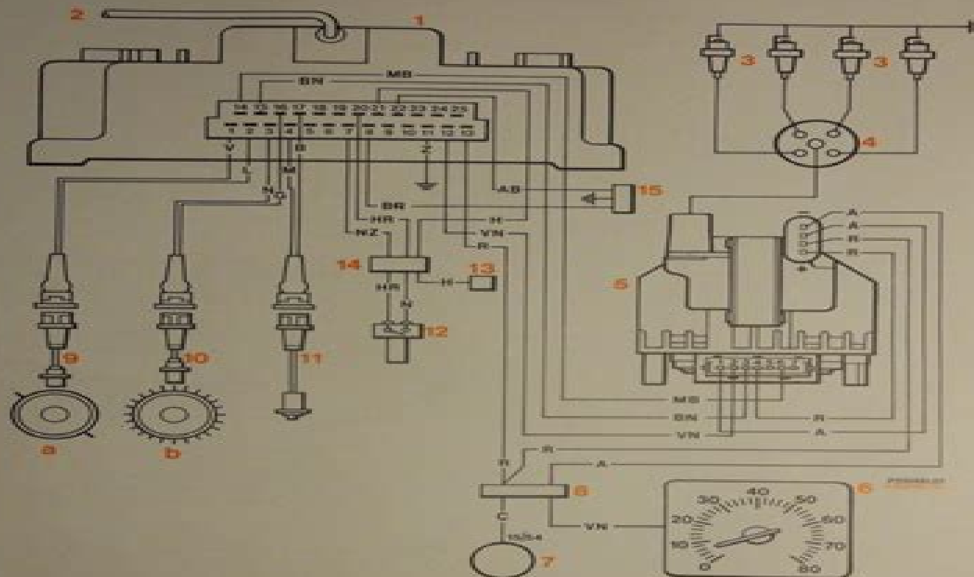
MICROPLEX IGNITION SYSTEM WIRING DIAGRAM
