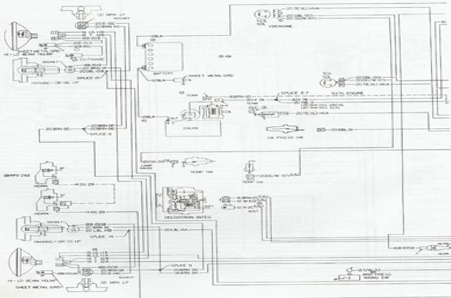
Typical 1973 through 1976 engine compartment and front lighting
