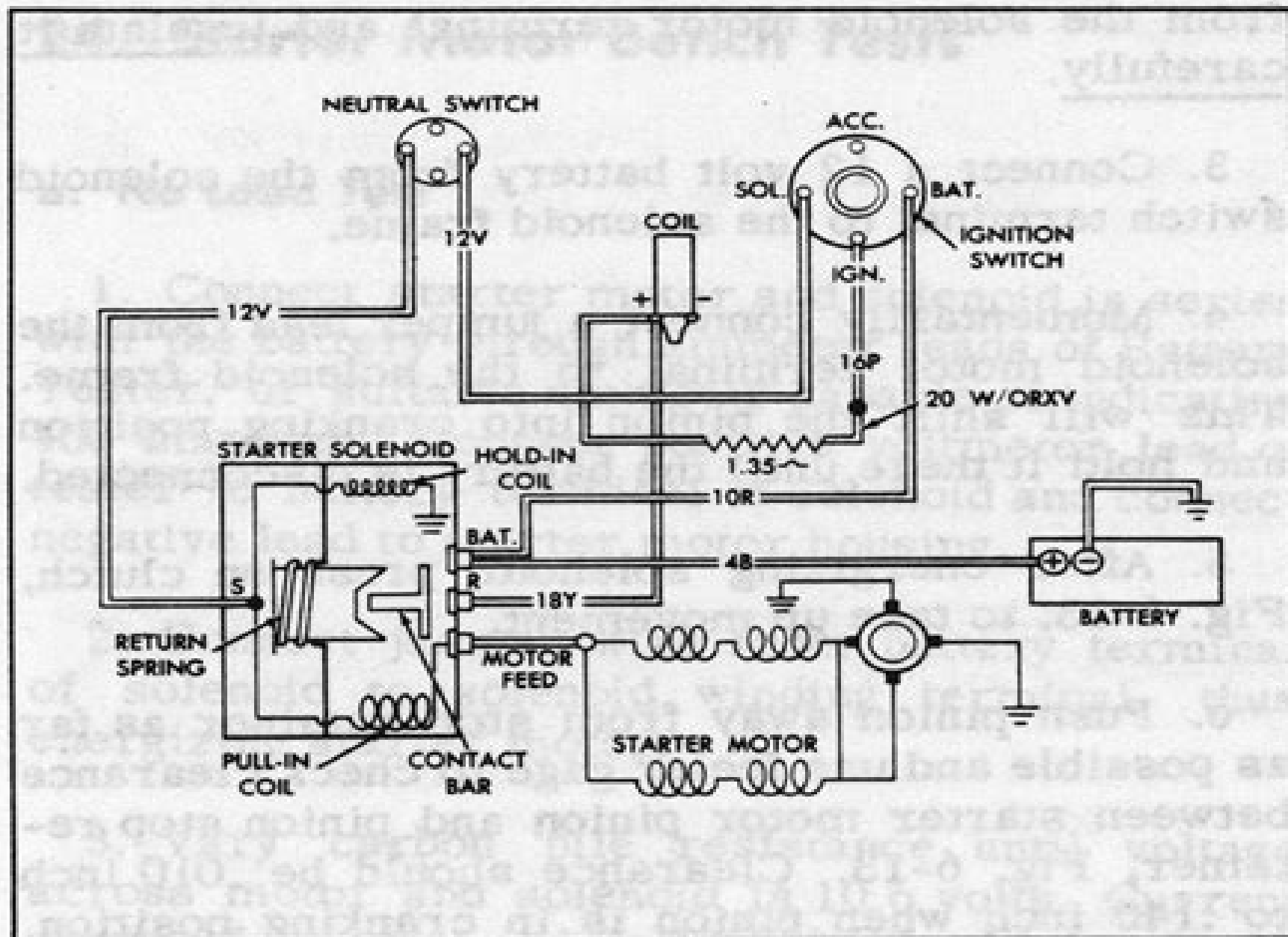
Fig. 6-10 Starting System Circuit
