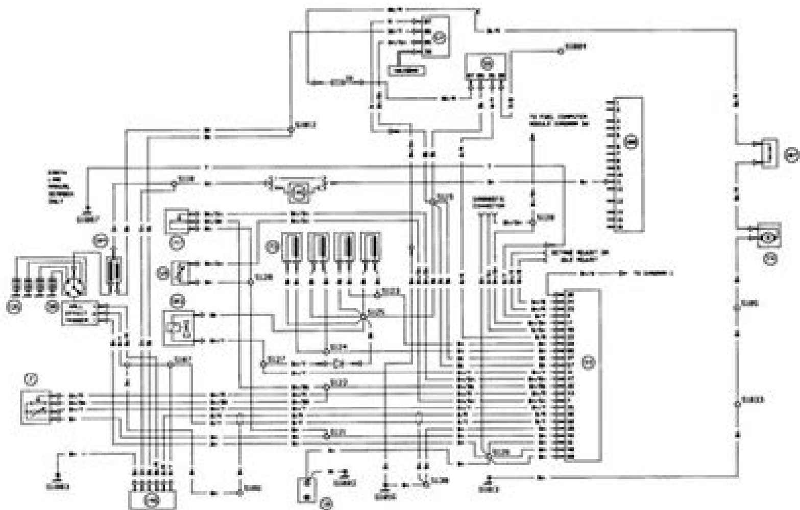
Diagram 4. 2.0 ES fuel injection and ignition. Models from 1987 to May 1989
