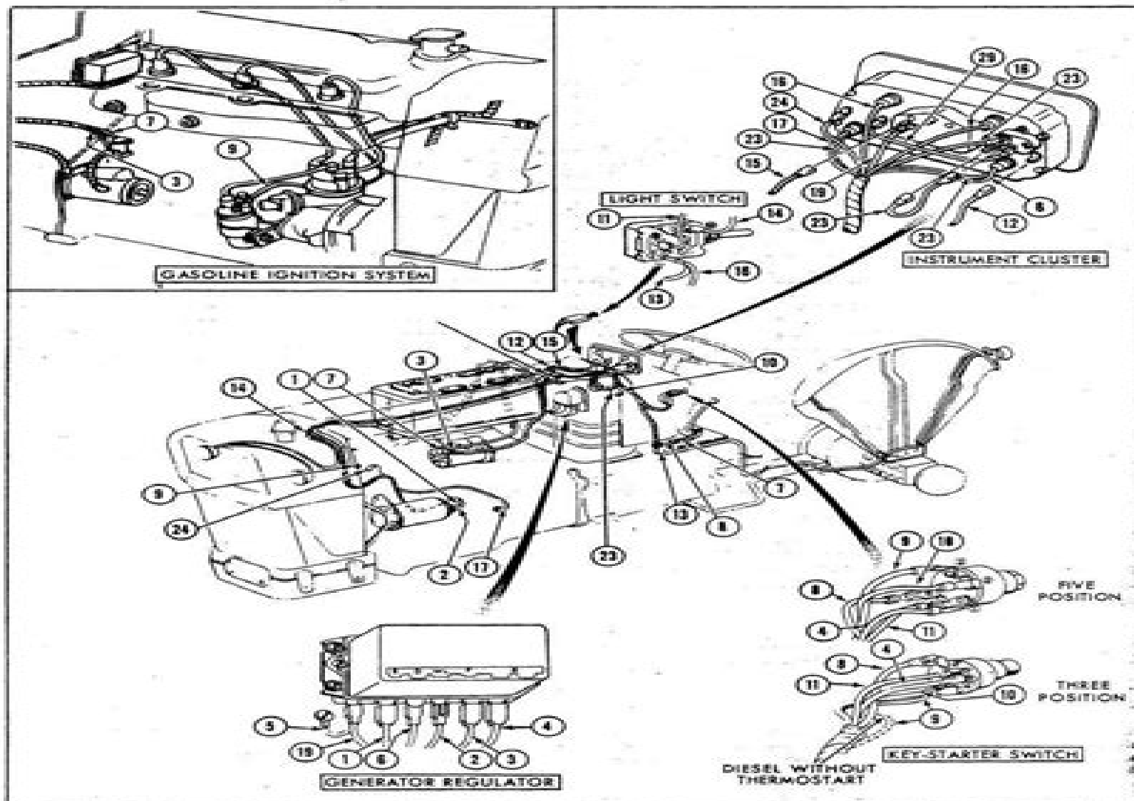
Figure 7 Circuit Descriptions—Tractors with "C" Prefixed Serial Numbers
