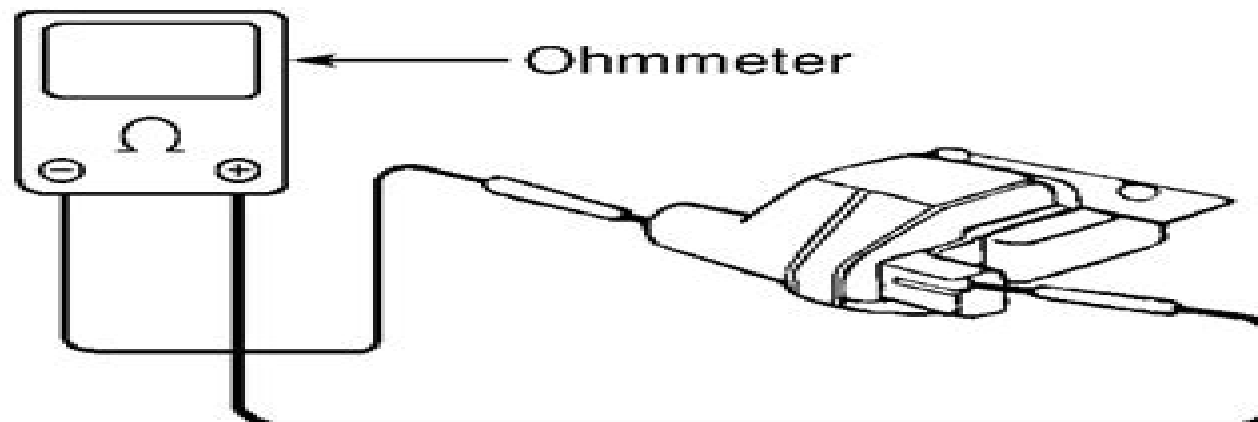
CHECKING SECONDARY RESISTANCE
