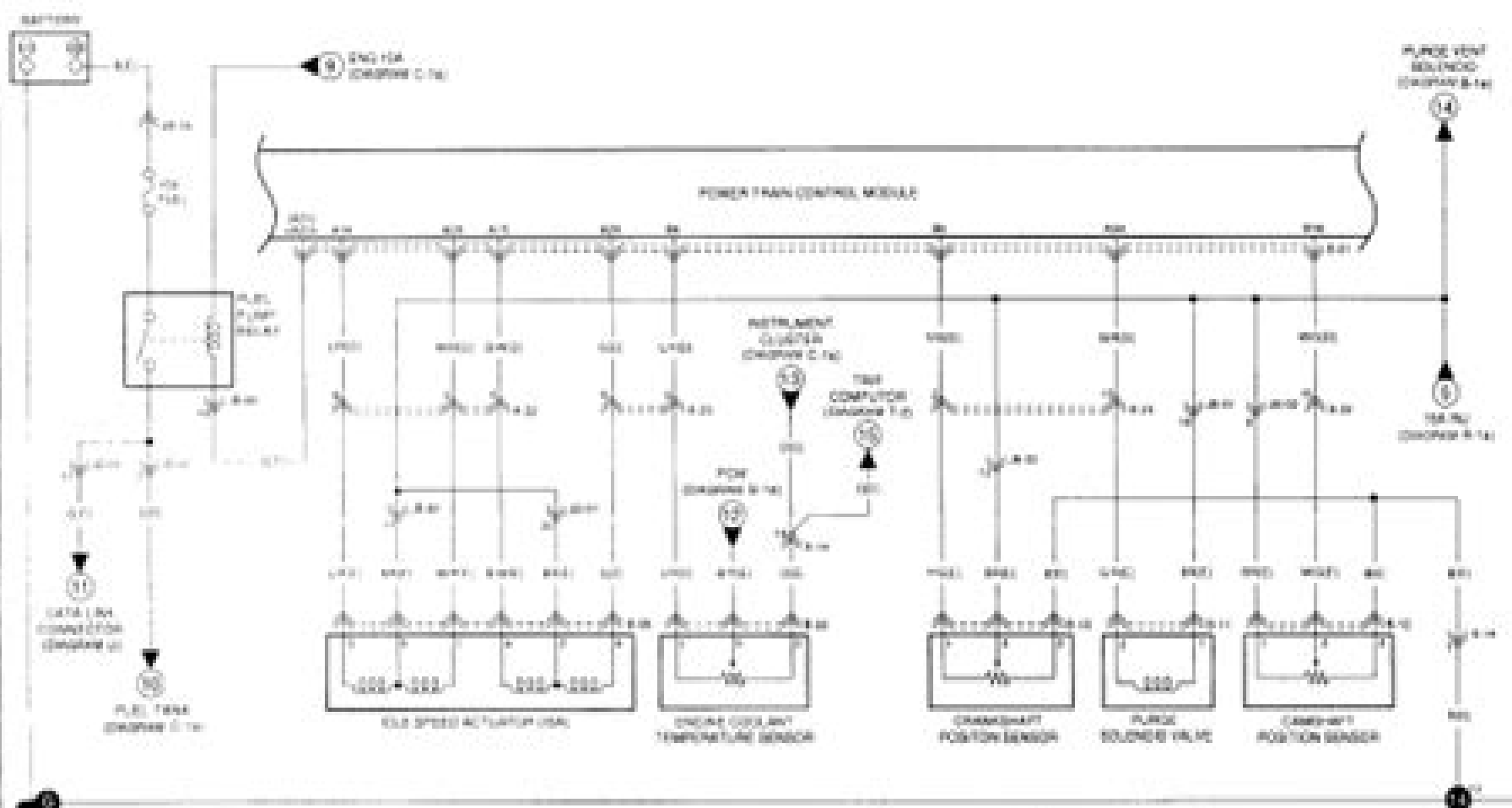
B-1b POWER TRAIN CONTROL MODULE (B)
