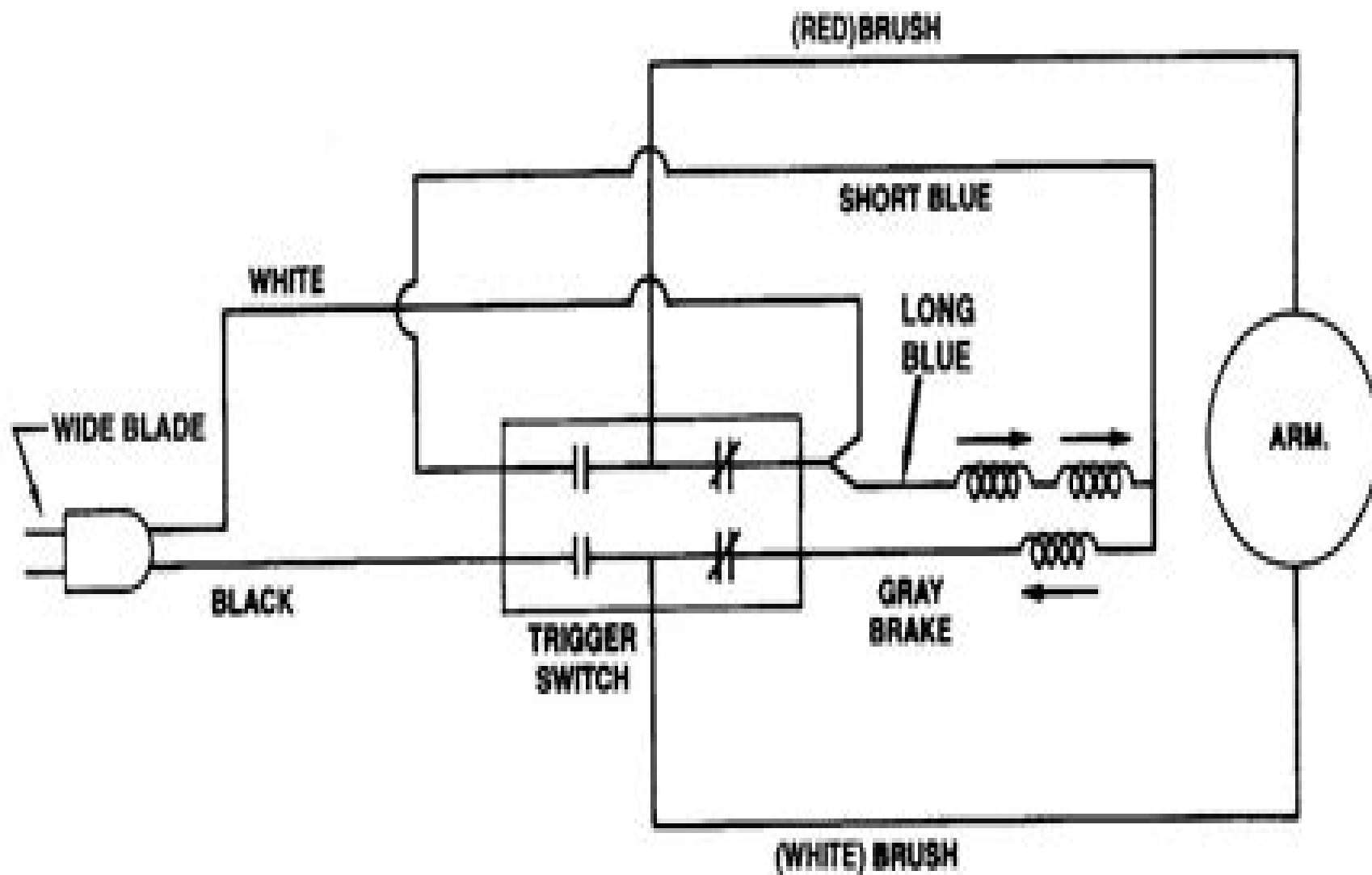
CIRCUIT DIAGRAM
