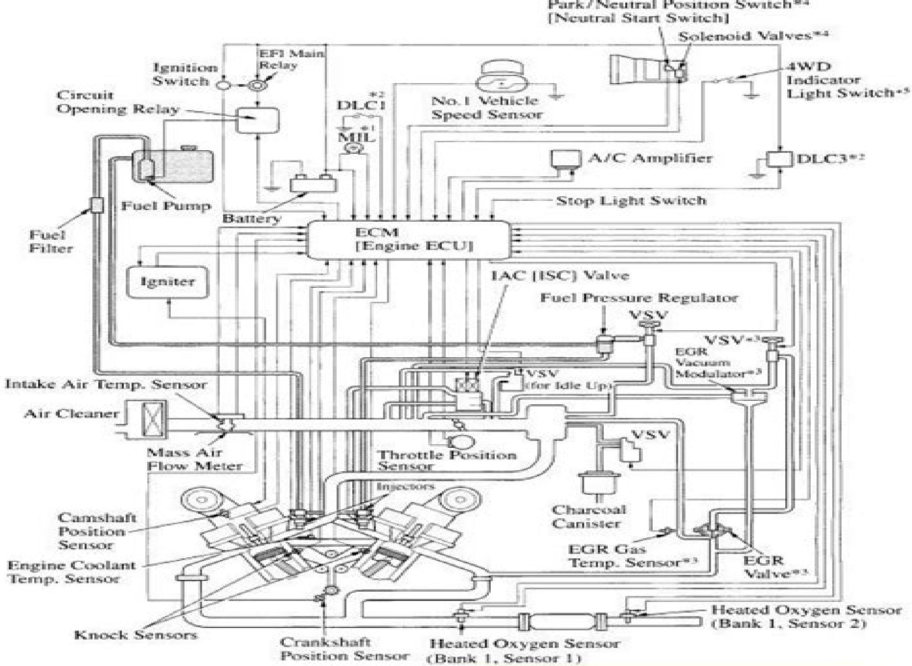
1998 Toyota T100 Engine Control System Diagram
