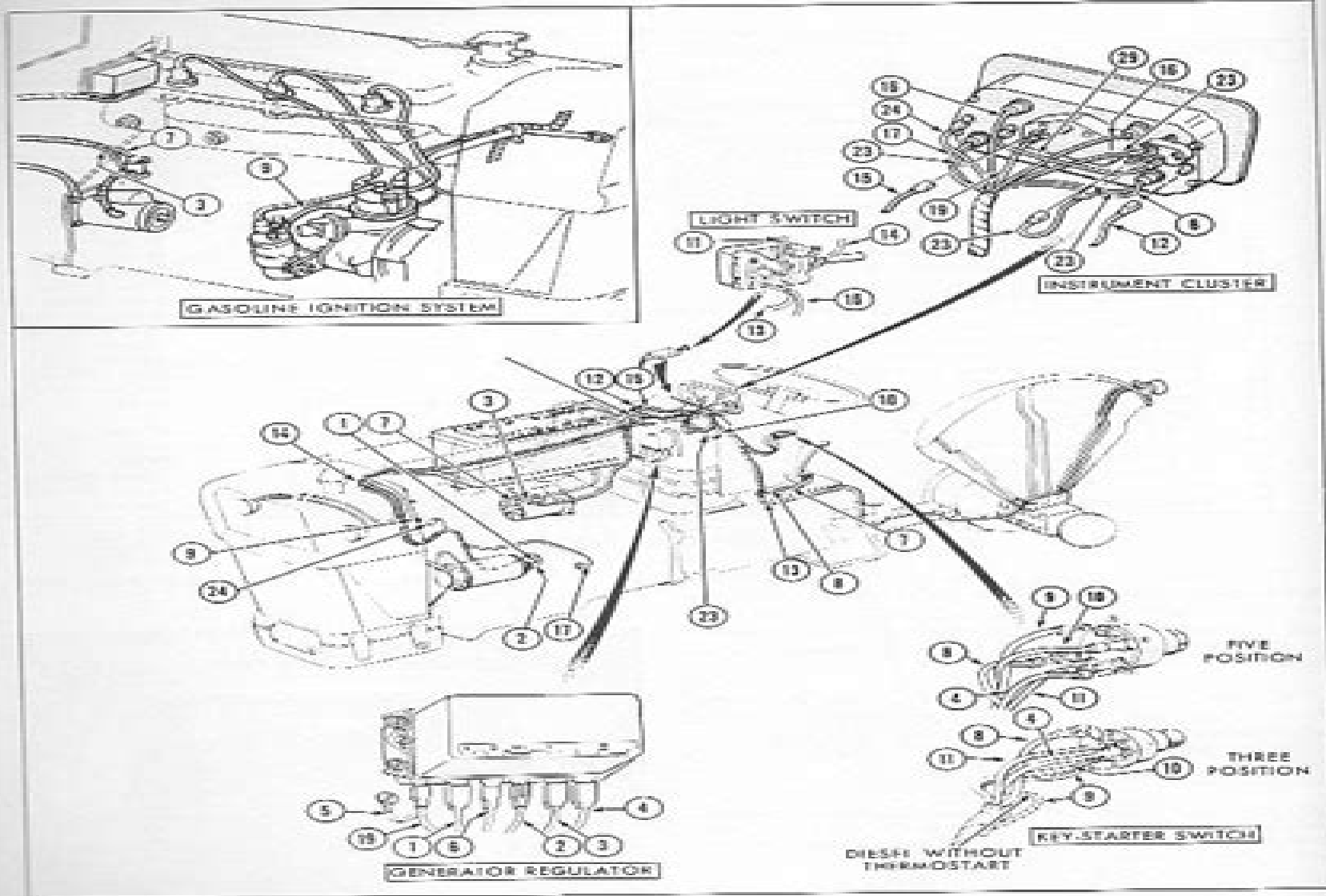
Figure 7 Circuit Descriptions—Tractors with "C" Prefixed Serial Numbers
