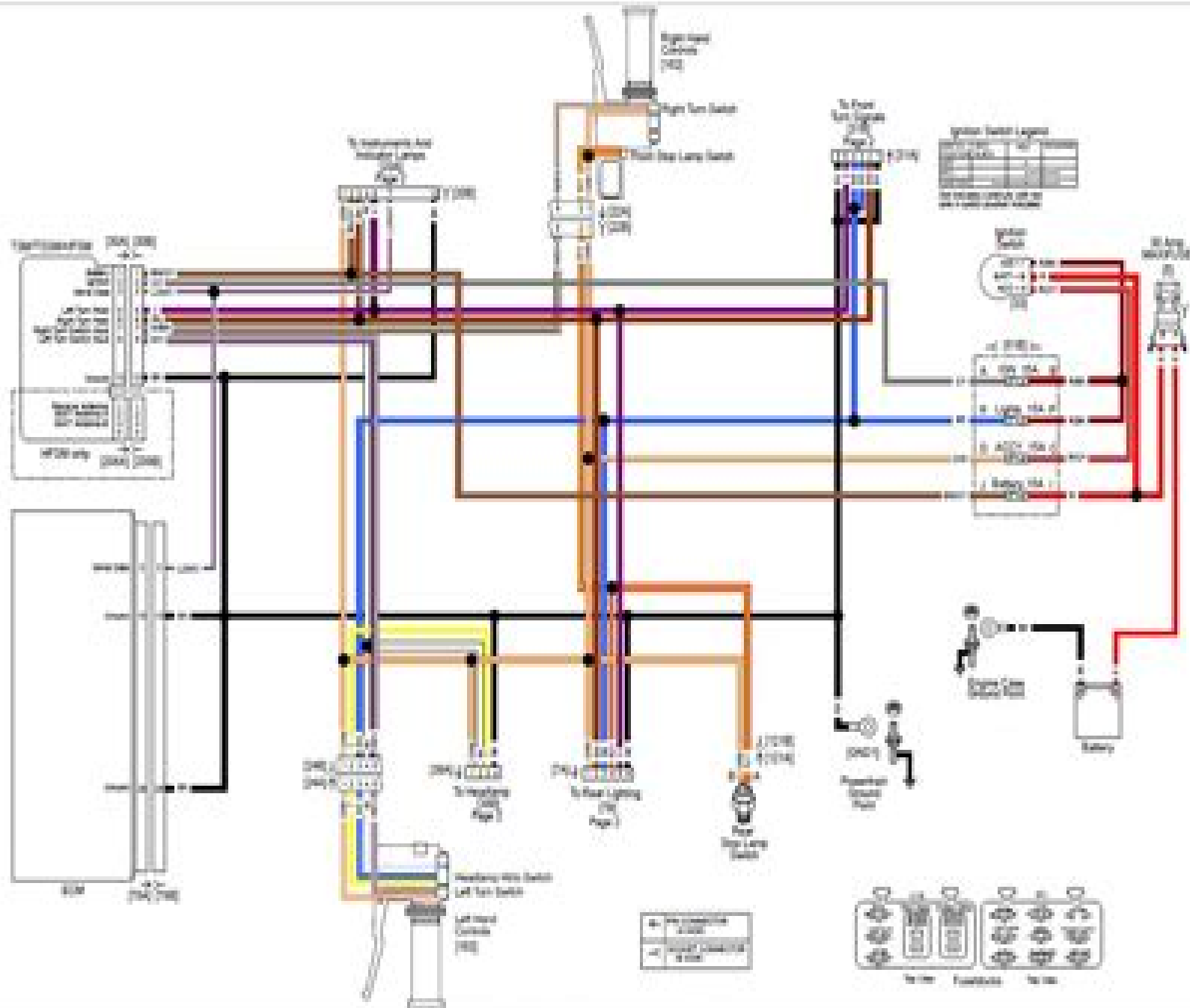
Figure 6-14. Lights (1 of 2) (00) 2000 Spectator DCM and MFL Module
