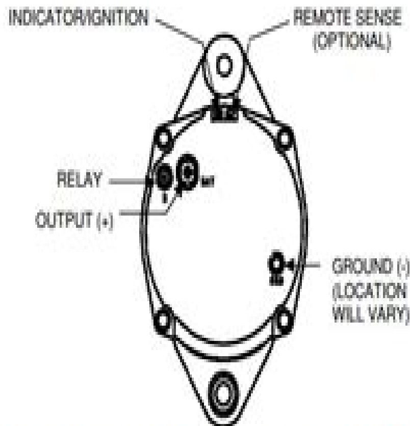
21SI & 22SI REMOTE SENSE 2-TERMINAL REGULATOR
