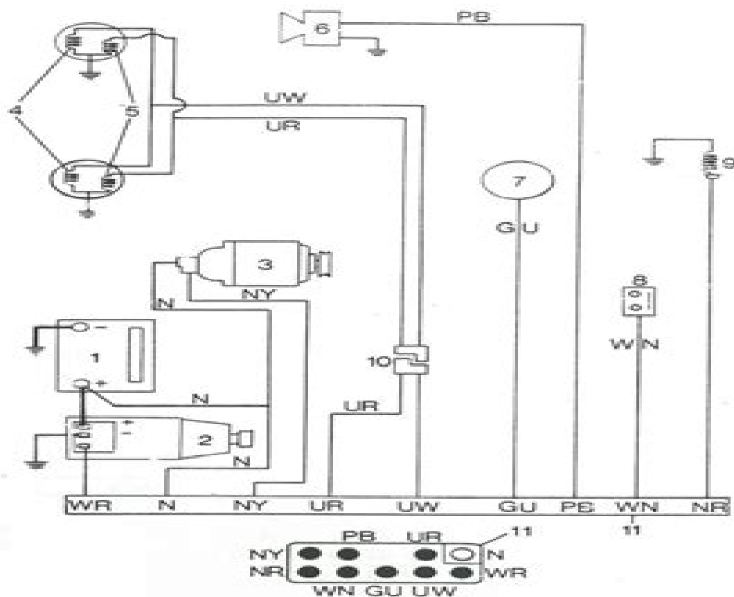
Figure H129 ENGINE HARNESS For tractors with an alternator, from the following serial numbers:
