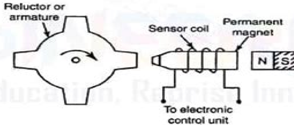
Figure 2.37 Magnetic pickup control unit
