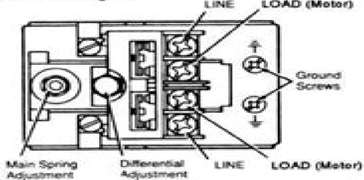
Connection Diagram
