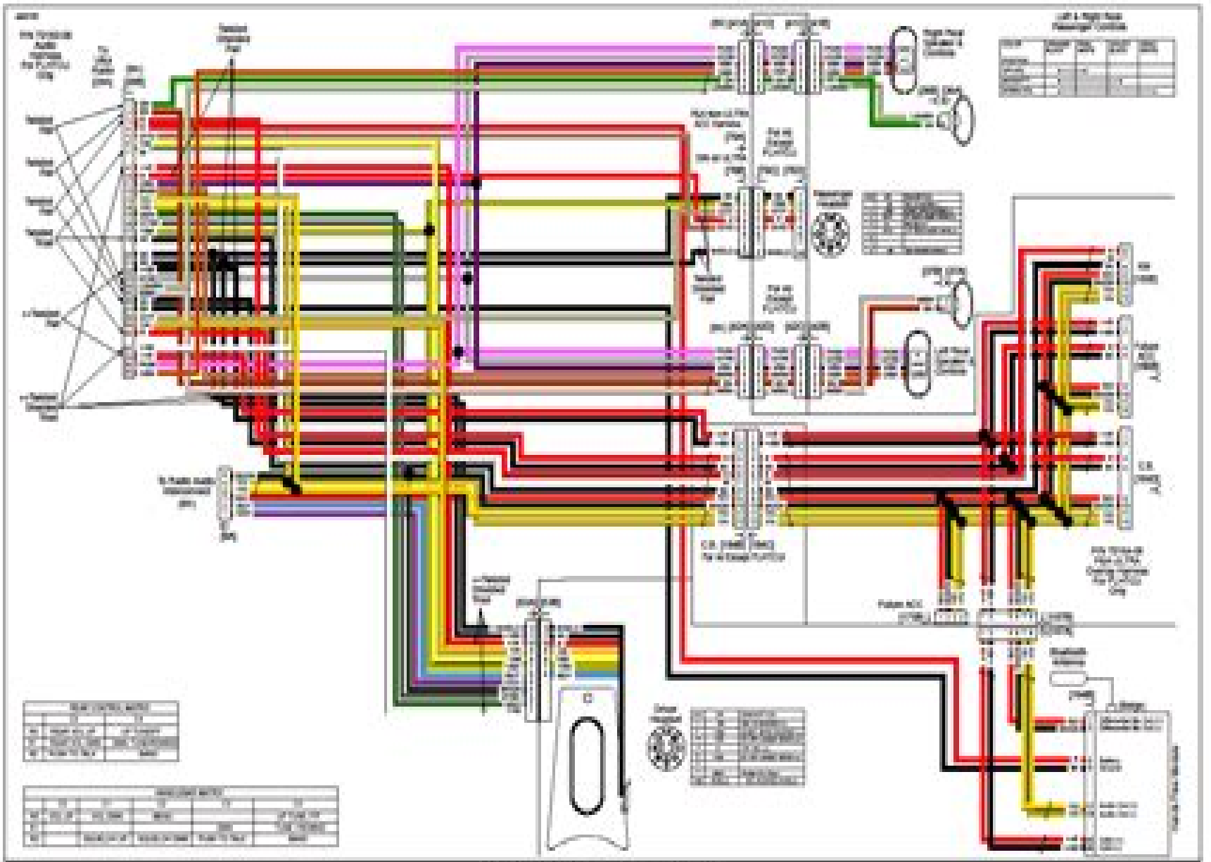
Figure 5-21 2000 Ultra Audio Interconnect Harness
