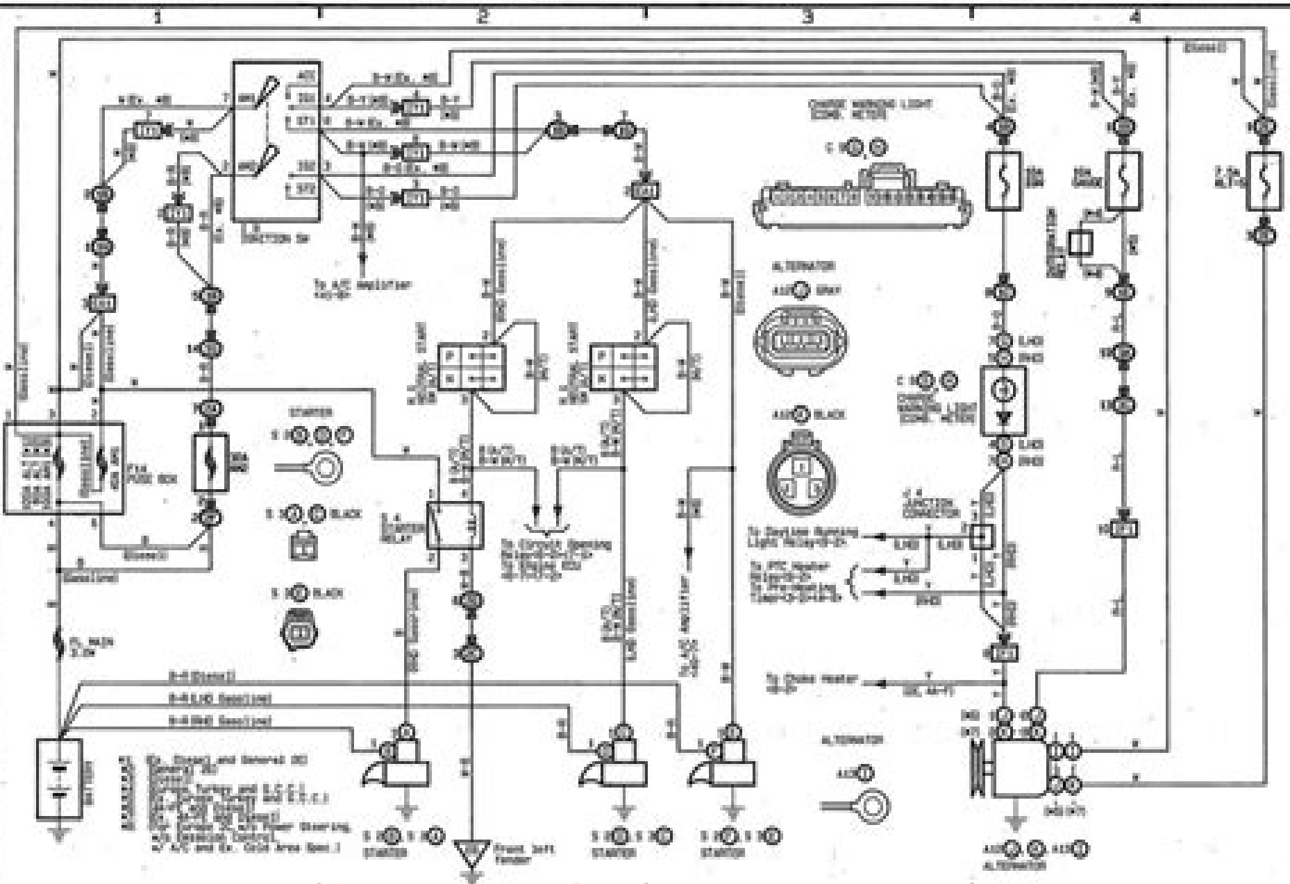
Wiring diagram for charge and start
