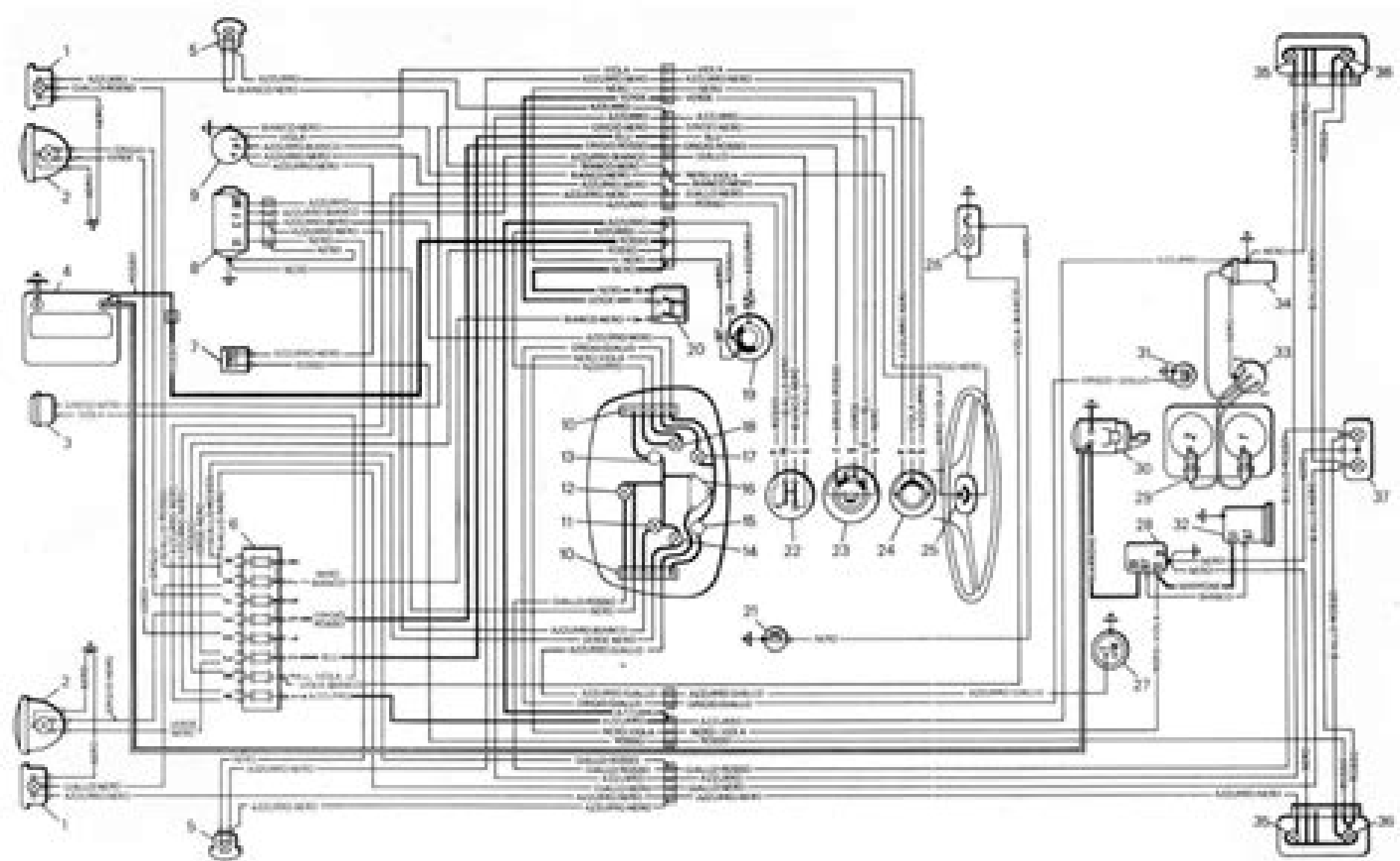
FIG 13:1 Wiring diagram for Fiat 126
