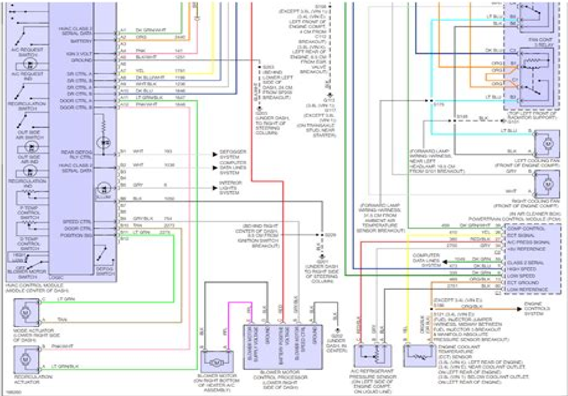
Fig 2: Manual A/C Circuit
