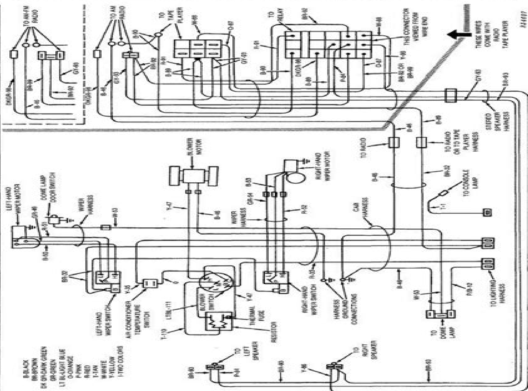
Fig. 28. SOUND-GARD Body Harness Connections
