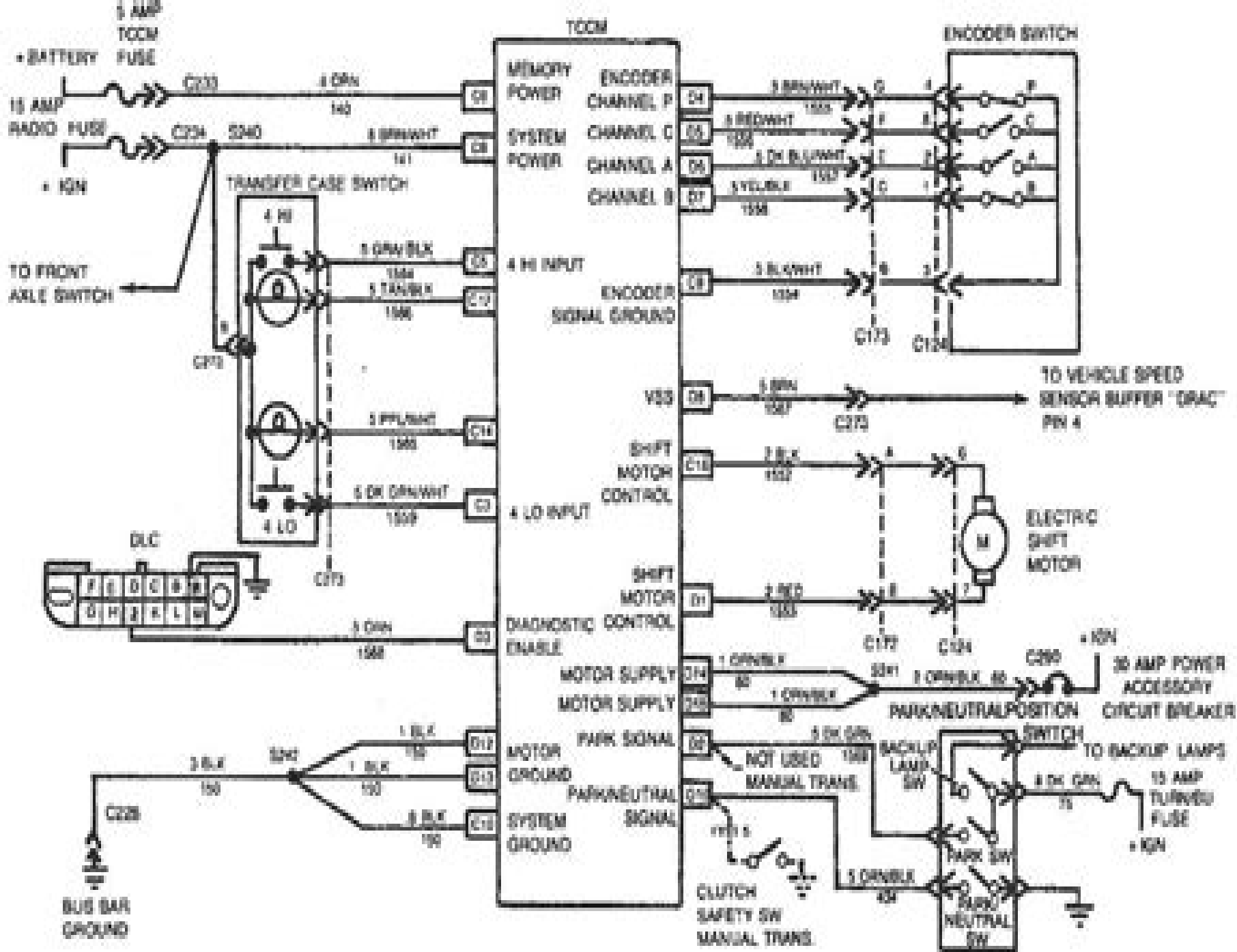
Fig. 4 Electronic Transfer Case Wiring Diagram
