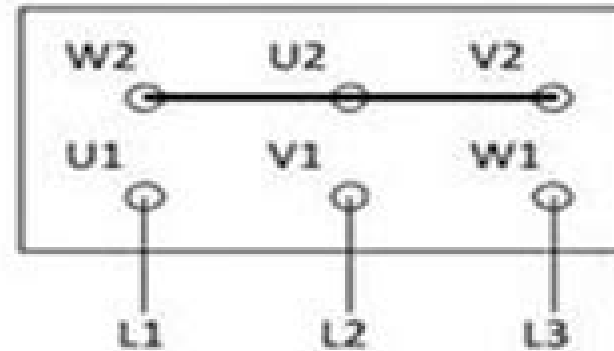
Terminal Connections
