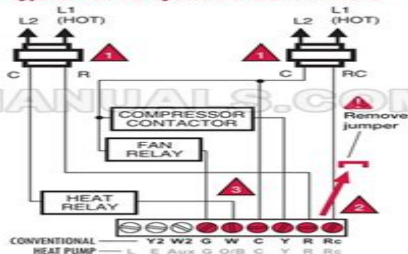
Typical 1H/1C system: 2 transformers
